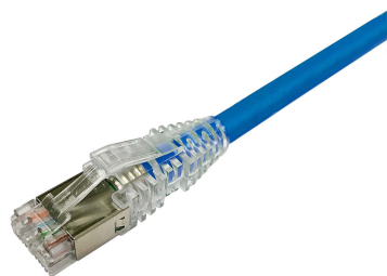
NPC RJ45 Patch Cord, category 6A, S/FTP, LSZH, blue
